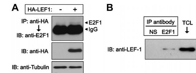
Fig. 3. Association between LEF-1 and E2F1 in vivo. (A) HEK293T cells were transfected with HA-tagged LEF-1 (3 \mu g) as indicated. At 40 h post-transfection, cells were harvested for anti-HA immunoprecipitation (IP). LEF-1-associated E2F1 was revealed by anti-E2F1 immunoblotting (upper panel). The protein expression was confirmed by anti-HA or anti-LEF-1 immunoblotting (IB) with the total cell lysates (middle and lower panels). (B) HEK293T cells were harvested for anti-E2F1 or control anti-none specific (NS) immunoprecipitation (IP). E2F1-associated LEF-1 was revealed by anti-LEF-1 immunoblotting. “TCL” represented “total cell lysates” as control (upper panel).
