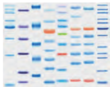
Western Blot
